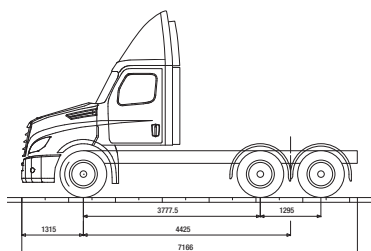
DAY CAB
